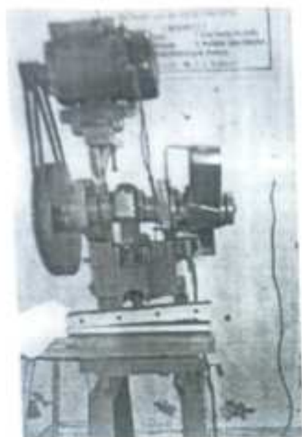
Spiral Punching Machine
